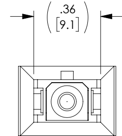
SC PLUG
