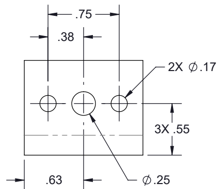
BRACKET MOUNTING PATTERN
